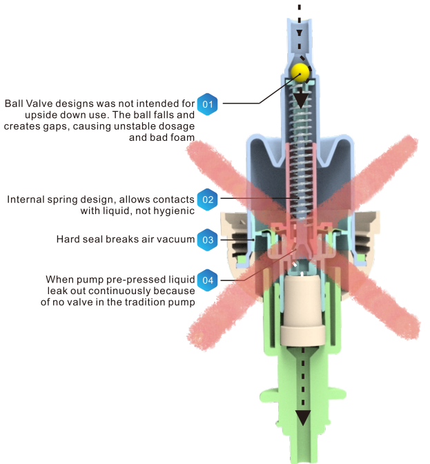
Traditional Pump Not Intended For Dispenser Use
