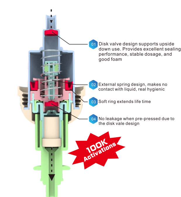
Faner New Pump Design For Dispenser Use
