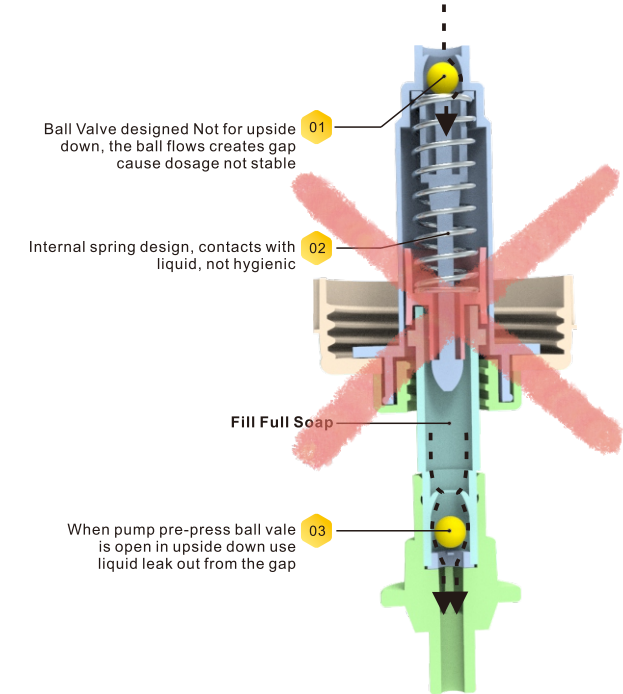
Traditional Pump Not Intended For Dispenser Use
