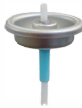
MODEL:AF-75 Metered Valve Ø1 inch, 75~85mcl Stem: 2.8mm, metal/plastic
