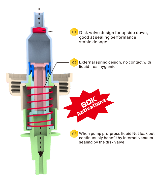
Faner New Pump Design For Dispenser Use
