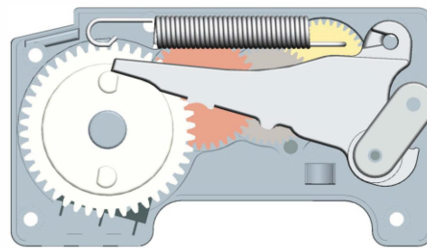
Special spring mechanism, supplying consistent pumping force, for stable spraying performance
