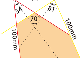
Sensing area V-type infrared emission to prevent interference
